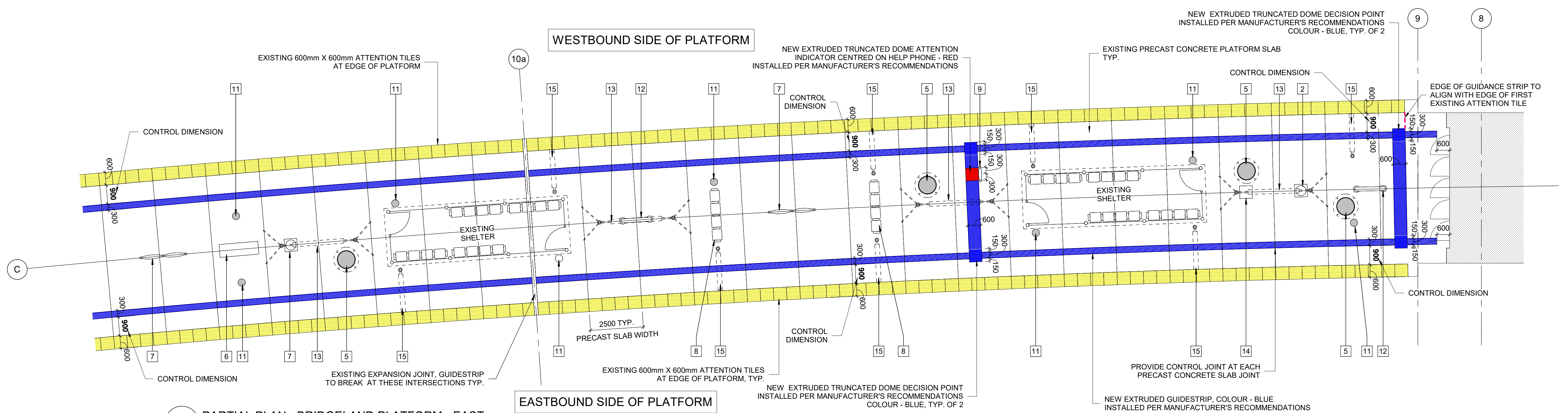
2 PARTIAL PLAN - BRIDGELAND PLATFORM - EAST A102 Scale: 1 : 100
