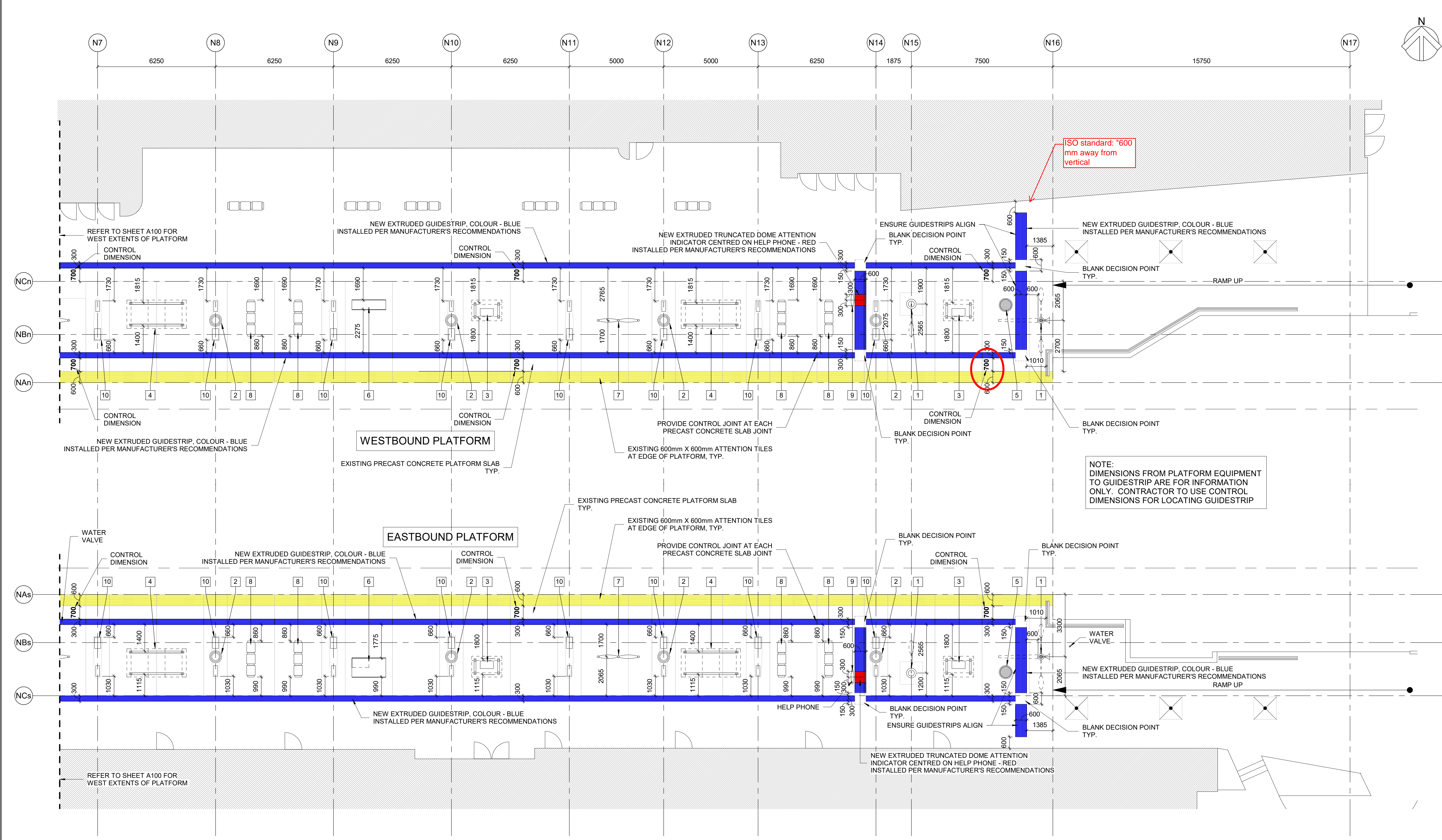
1 CITY HALL PLATFORM - EAST A101 Scale: 1 : 100
